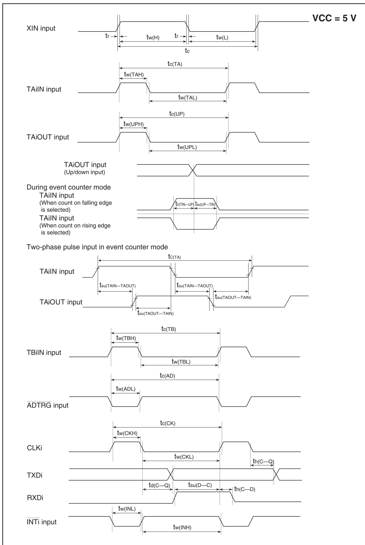
Figure 5.21 Timing Diagram
